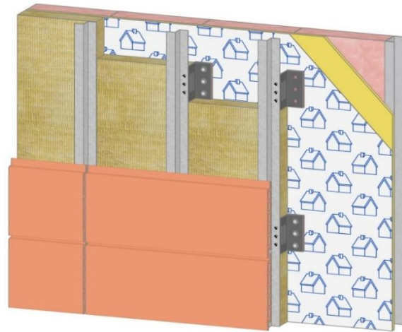
Figure 8 – Stainless Steel Clips
