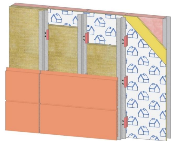
Figure 10 – Fiber Glass Clips
